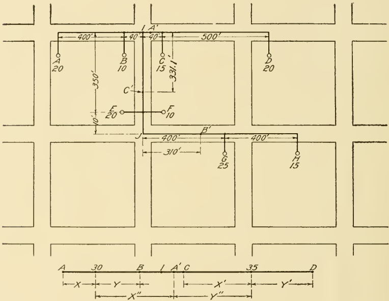
Fig. 10. Diagram to Determine Feeding Point
